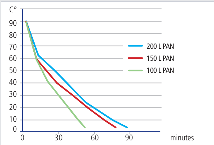
SAMPLE CHILLING TIME DIAGRAM (product: vegetable soup)
